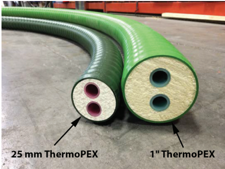
1" ThermoPEX provides superior insulating properties; 25 mm ThermoPEX is more flexible and easier to handle
